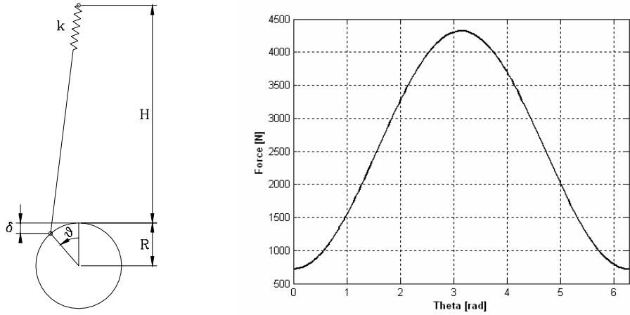
Figure 1. Scheme of the harmonic exciting system (left); spring force vs engine angular position (right).
