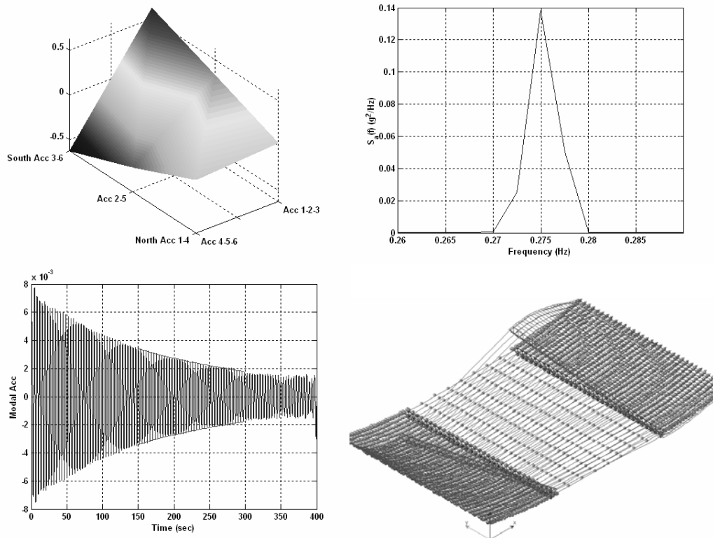
Figure 7. First mode dynamic properties. Test n. EXCB06; experimental frequency f_{exp} = 0,275 Hz; experimental damping ratios: \xi_{large\ amplitudes} = 3,0\% - \xi_{mean\ amplitudes} = 2,5\% - \xi_{small\ amplitudes} = 2,3\% ; FEM theoretical frequency f_{theor} = 0,274 Hz.
