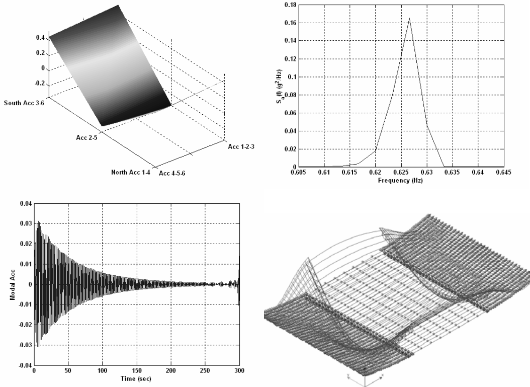
Figure 8. Fifth mode dynamic properties. Test n. EXCB17; experimental frequency f_{exp} = 0,627 Hz; experimental damping ratios: \xi_{large\ amplitudes} = 4,5\% - \xi_{mean\ amplitudes} = 3,7\% - \xi_{small\ amplitudes} = 3,1\% ; FEM theoretical frequency f_{theor} = 0,54 Hz.
