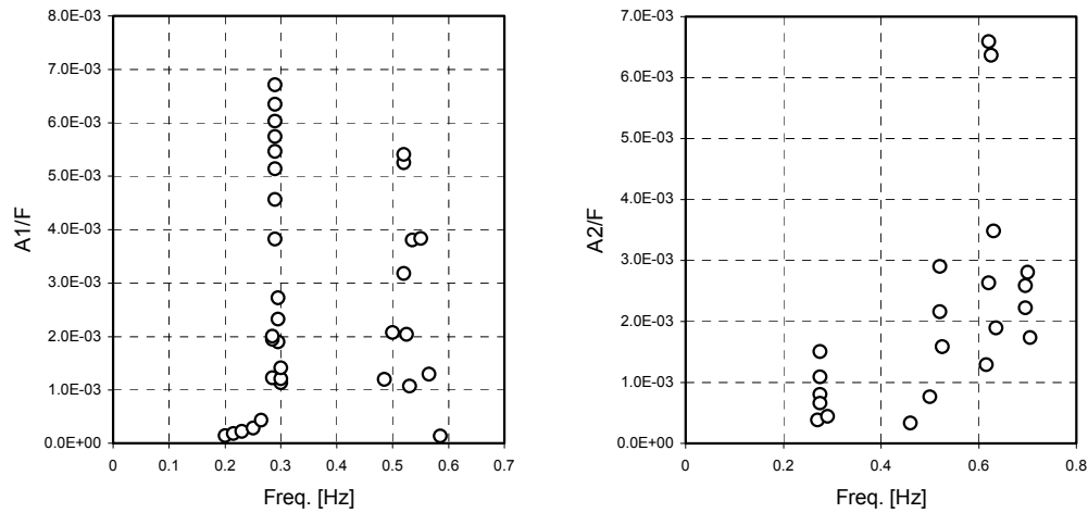
Figure 5. Dynamic response ratio A/F vs excitation frequency: force in EXC A (left) and EXC B (right).
