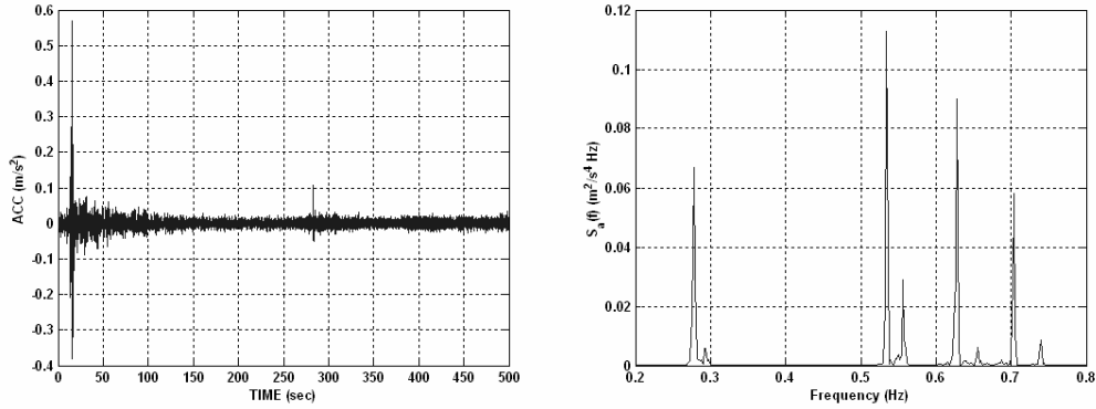
Figure 4. Acceleration time history (left) and PDSF (right): impulse in EXC B - sensor ACC 3.
