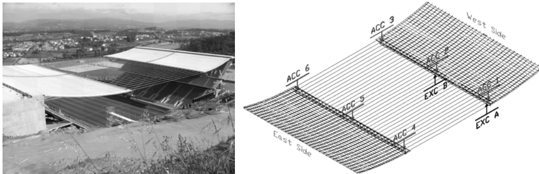
Figure 3. Stadium roof view (left); accelerometers and exciting system position (right).
