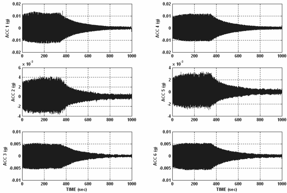
Figure 6. Typical record of acceleration time series (Test n. EXCA22, force in EXCA, freq. 0.29 Hz).
