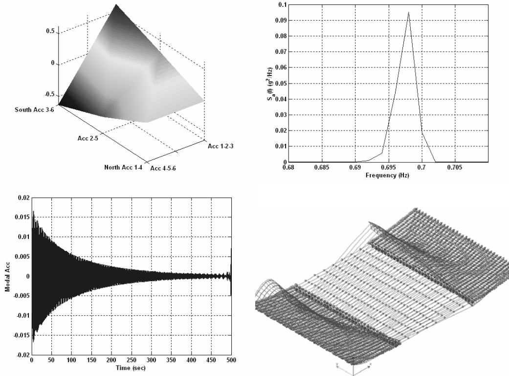
Figure 9. Tenth mode dynamic properties. Test n. EXCB21; experimental frequency f_{exp} = 0,698 Hz; experimental damping ratios: \xi_{large\ amplitudes} = 2,2\% - \xi_{mean\ amplitudes} = 1,6\% - \xi_{small\ amplitudes} = 1,3\% ; FEM theoretical frequency f_{theor} = 0,678 Hz.
